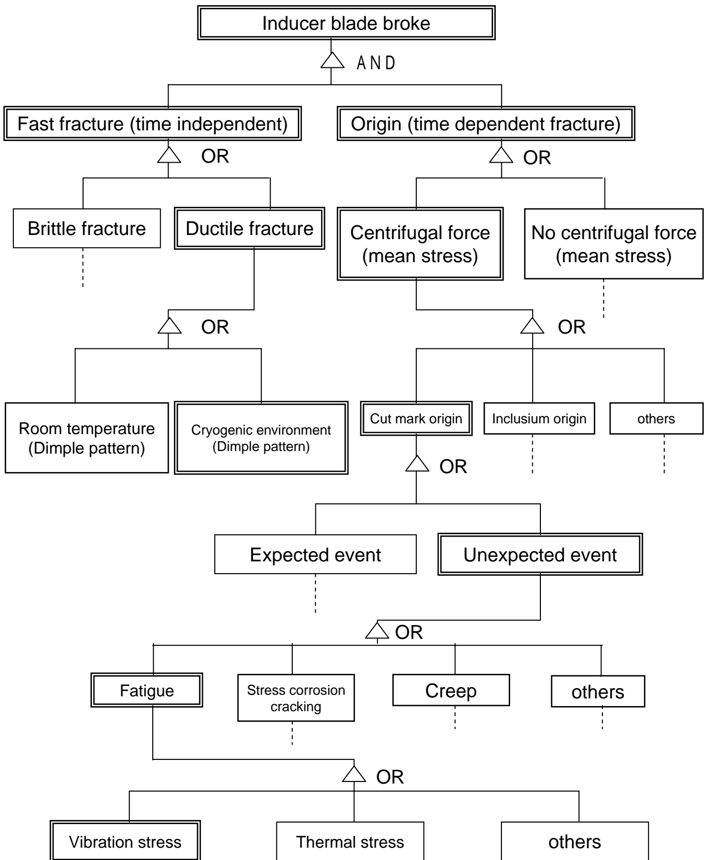
Fig.2 Fault tree diagram for mode, mechanism and process of fracture
